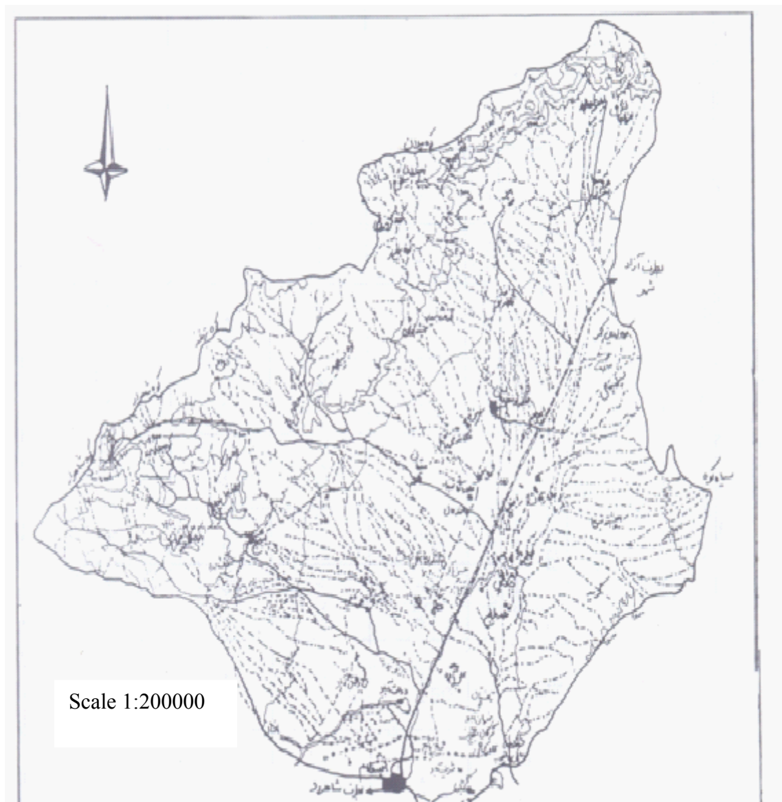
Figure2. Bastam watershed
